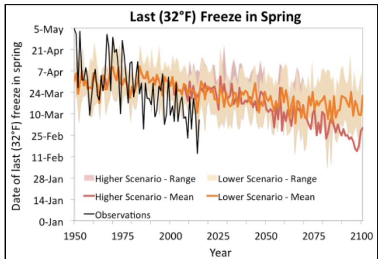
Figure 16: Projections of date of last freeze (32°F) in spring for a lower emissions scenario (orange line) and higher scenario (red line). Shaded areas indicate the range of model projections, and colored lines indicate the average of all models. Black line shows historical observations.
